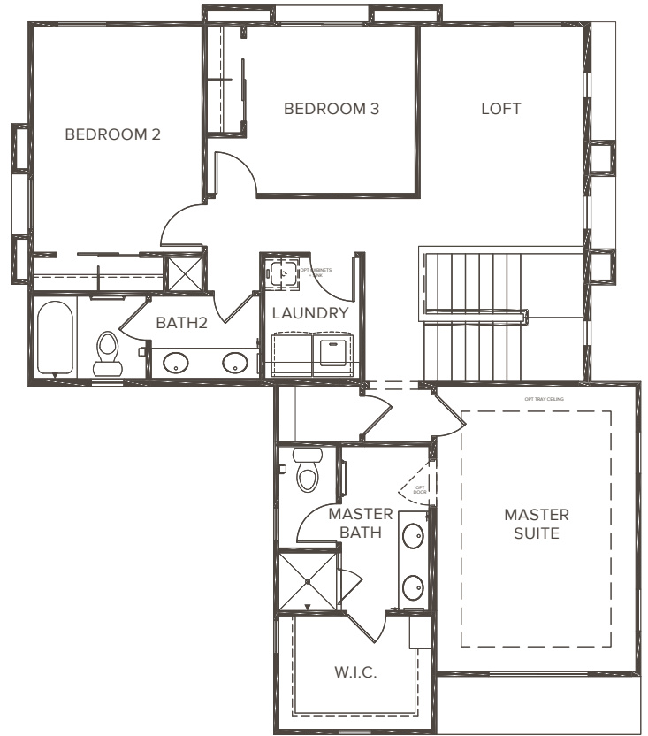
SECOND FLOOR
